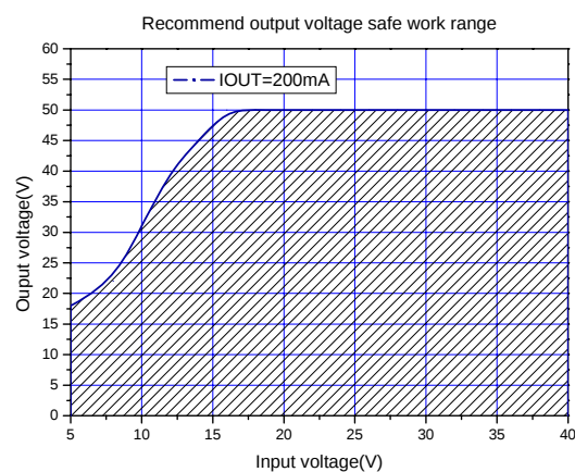
Figure6.Max output voltage(IOUT=200mA)
