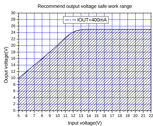
Figure8.Max output voltage(IOUT=400mA)
