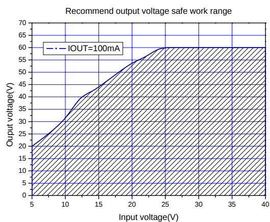
Figure5.Max output voltage(IOUT=100mA)
