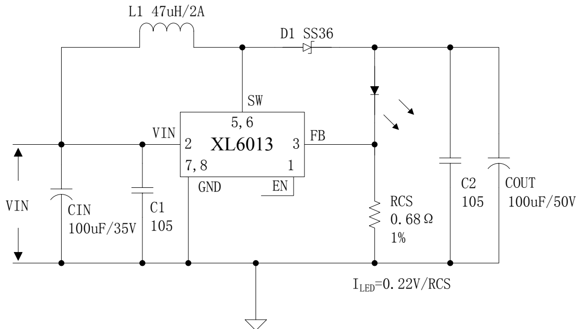
Figure11. XL6013 System Parameters Test Circuit (VIN=5V~30V, IOUT=320mA)
