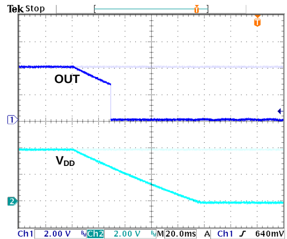
Figure 14. Power-Down OUT Timeout Waveforms for -V_{TH}=2.7V
