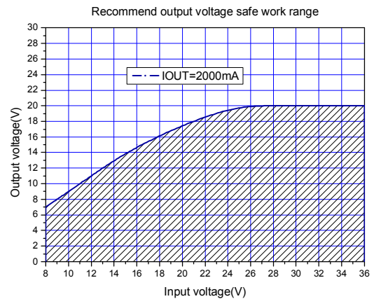
Figure15.Max output voltage(IOUT=2000mA)
