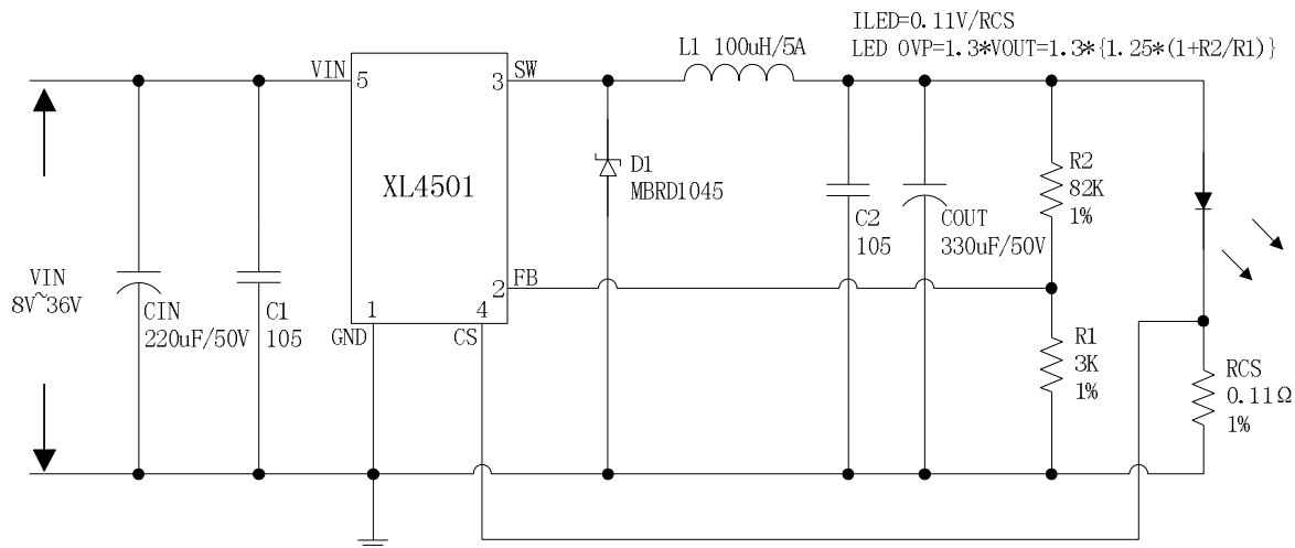
Figure24. XL4501 System Parameters Test Circuit (VIN=8V~36V,IOUT=1000mA)
