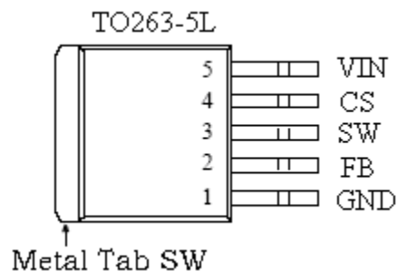
Figure2. Pin Configuration of XL4501 (Top View)
