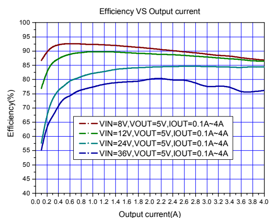
Figure8. Efficiency Curve
