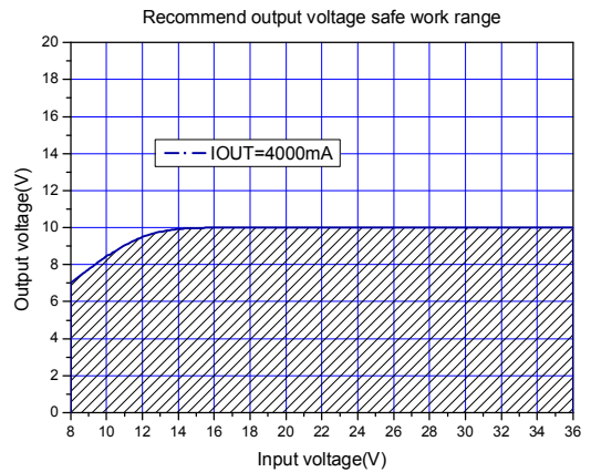
Figure17.Max output voltage(IOUT=4000mA)
