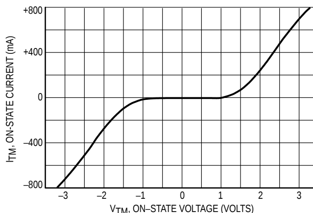
Figure 2. On-State Characteristics
