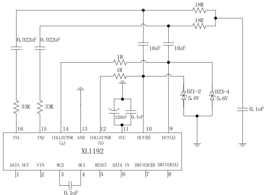
Figure3. XL1192 Typical Application Circuit (No external transistor)
