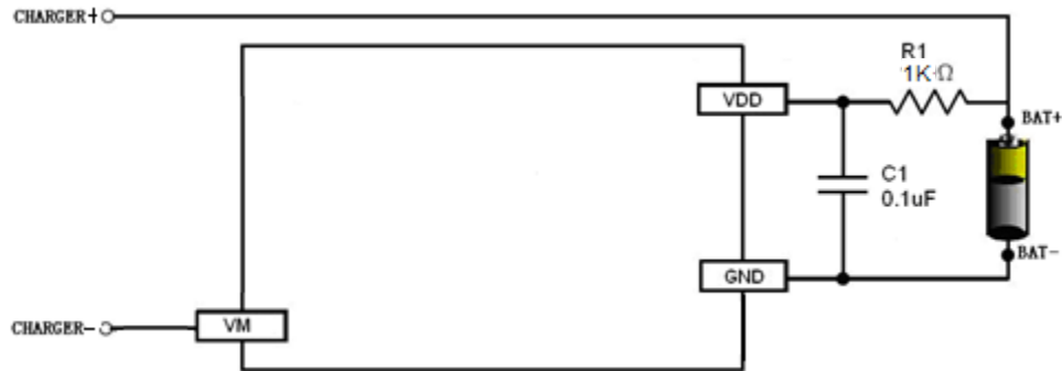
Fig 6 XB7608A in a Typical Battery Protection Circuit
