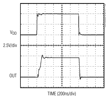
POWER-UP DELAY
