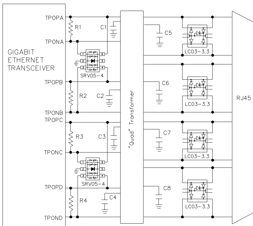
Figure 10 - Gigabit Ethernet Protection for Bellcore 1089 Intra-Building Protection
